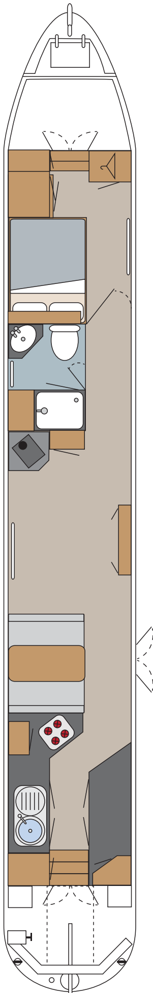
Example 58ft layout
